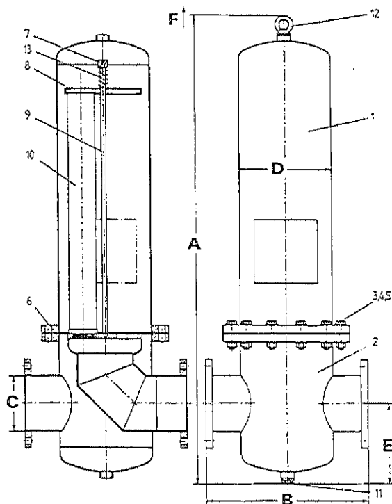
Multi-element with ANSI flange connection
